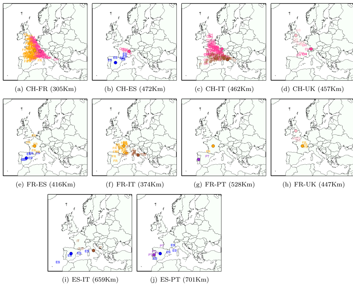
Figure 6: Ancestral location prediction error in real POPRES admixed individuals, stratified by the country of origin of each location. Letters are the inferred locations, and the shaded circles are the assumed true locations.
