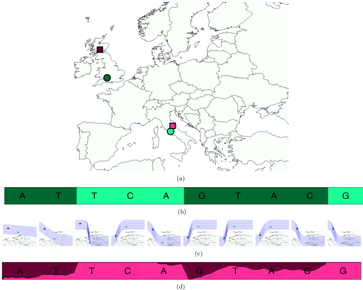
Figure 1: SPAMIX model for admixed individuals. (a) Example of haploid individual with two ancestry locations in Europe (circles denote the true ancestry locations). (b) The admixture process induces segments of different ancestry backgrounds. (c) SPAMIX uses logistic gradients to describe allele frequencies as a function of geographic map to instantiate an admixture HMM for each pair of locations on a map. Each location on the map is associated to a particular allele frequency at all sites in the genome. (d) SPAMIX finds the location of ancestors on a map (denoted by squares in subfigure (a)) and the locus-specific ancestry at each site in the genome by maximizing the likelihood of genotype data.
