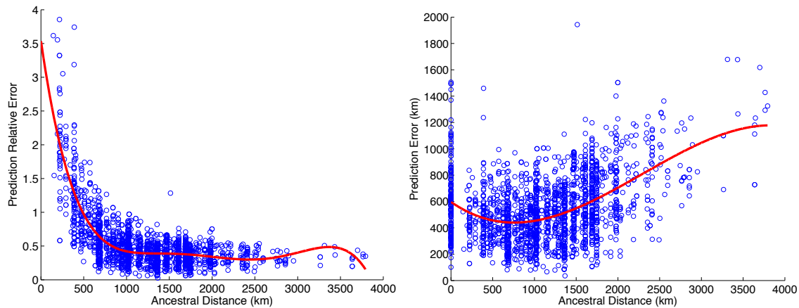
Figure 2: Ancestral location prediction error as a function of distance between ancestral locations in simulations over POPRES data. Left shows the prediction error normalized by the distance between the ancestral locations used in simulations and right plots the the prediction error. Simulations use the haploid model with 2 generations in the mixture.
