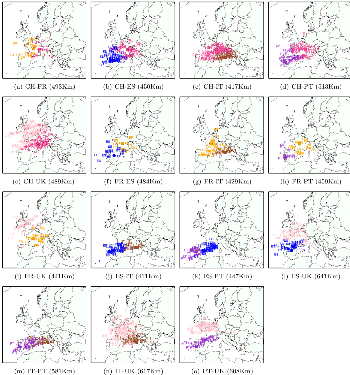
Figure 5: Ancestral location prediction error in simulations of European individuals with ancestry from two locations in Europe, stratified by the country of origin of each location (the country of origin is displayed in different colors). The assumed true locations are displayed by shaded circles. Results in parenthesis denote the average ancestral location prediction error across all simulations. In each simulation the reference data (used to estimate logistic gradients) is disjoint from data used to simulate admixed genomes (see Methods). The admixed genome is simulated as 4 generations ago, and SPAMIX diploid model is used for the inference. The number of simulated pairs can be found in Figure S4.
