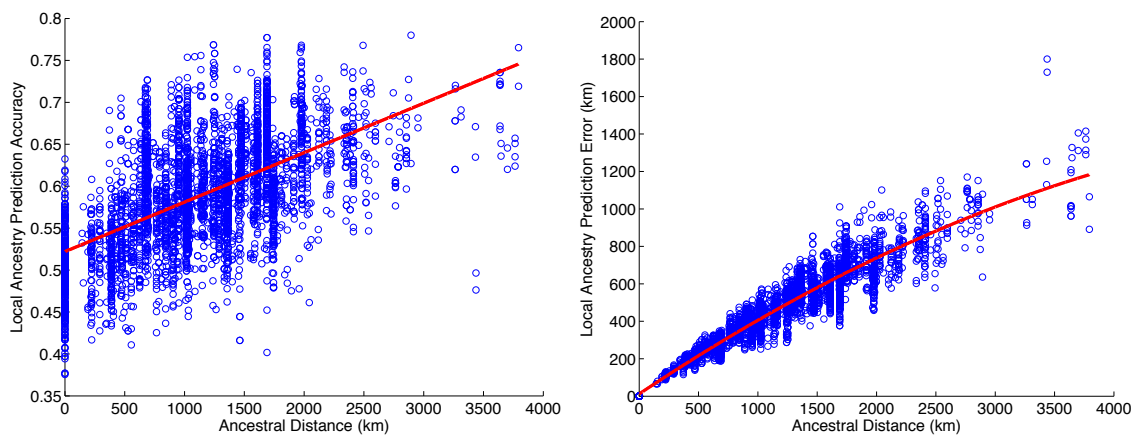
Figure 4: SPAMIX locus-specific ancestry prediction accuracy as function of distance between ancestral locations. Left displays the local ancestry prediction accuracy, defined as the percentage of all loci with correct assignment of ancestry. Right plot displays the average distance to true locations for each allele in the genome (local ancestry prediction error). Simulations use the haploid model with 2 generations in the mixture.
