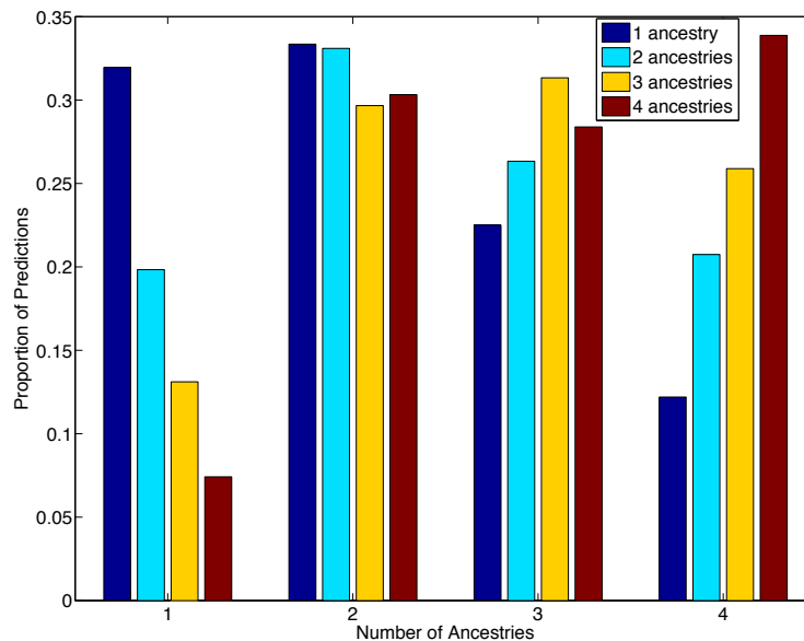
Figure 3: Inference of number of distinct ancestries using the Akaike information criterion (AIC). We simulated 1,000 admixed individuals with up to 4 distinct ancestry sources in Europe and used the AIC within the SPAMIX model to infer the number of ancestries. Figures show the proportion of inferred number of ancestries (y-axis) as function of number of simulated ancestries (x-axis) Although we observe a large variance in the number of predicted ancestries we note that the histogram is centered on the correct simulated number of ancestries thus suggesting that AIC could be employed to infer the number of distinct ancestors.
