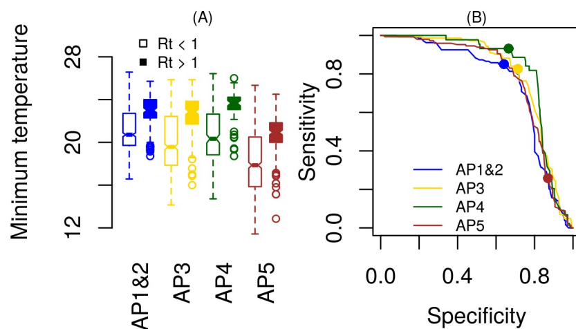
300 Figure 4. (A) boxplots of temperature values in weeks with R_t above or below 1. Each color corresponds to a different area of the city. (B) sensitivity-specificity plot of different cutoff points of temperature to discriminate weeks with R_t > 1 . Dots indicate the cutoff used (22C).
