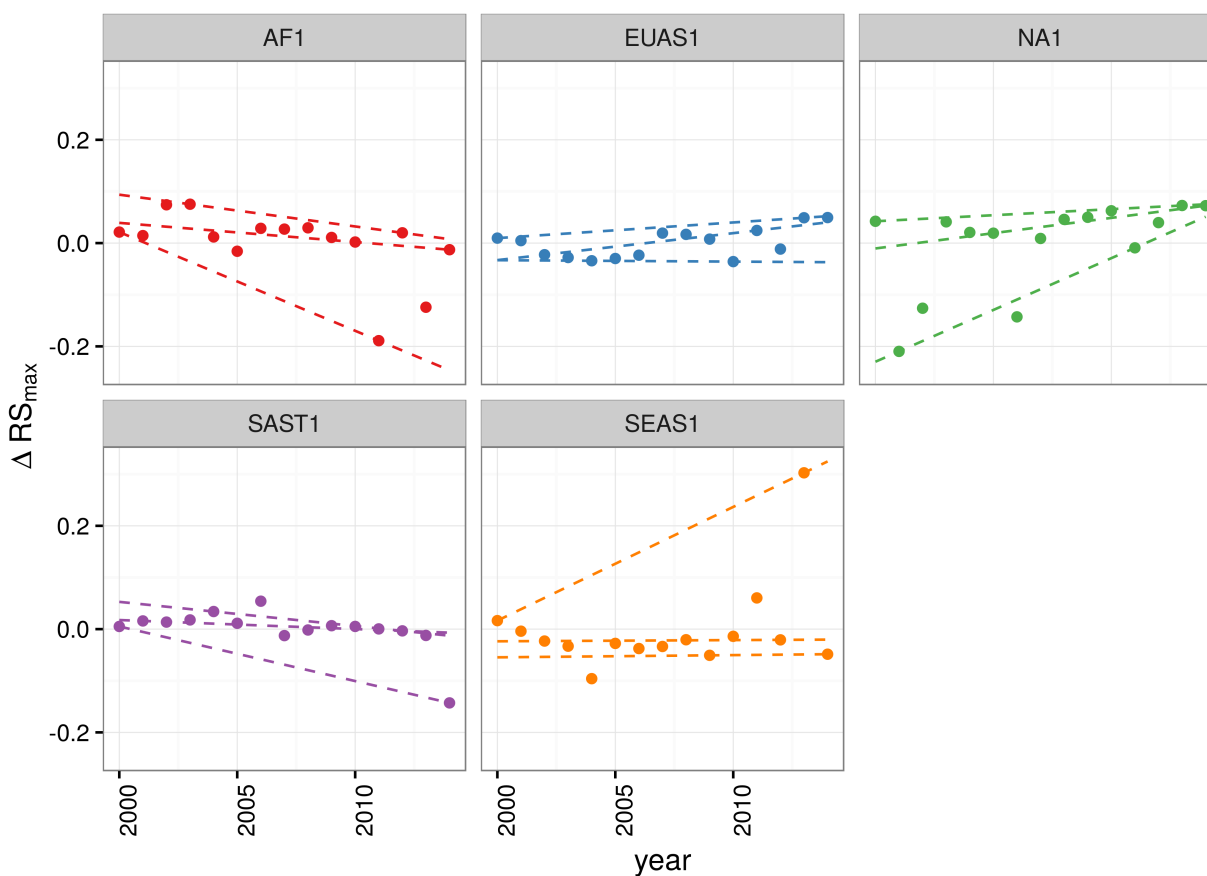
Figure 4: Largest patch fluctuations for regions with total forest area > 10^7 \text{km}^2 across years. The patch sizes are relative to the total forest area of the same year. Dashed lines are 90%, 50% and 10% quantile regressions, to show if fluctuations were increasing. The regions are AF1: Africa mainland, EUAS1: Eurasia mainland, NA1: North America mainland, SAST1: South America tropical and subtropical, SEAS1: Southeast Asia mainland.
