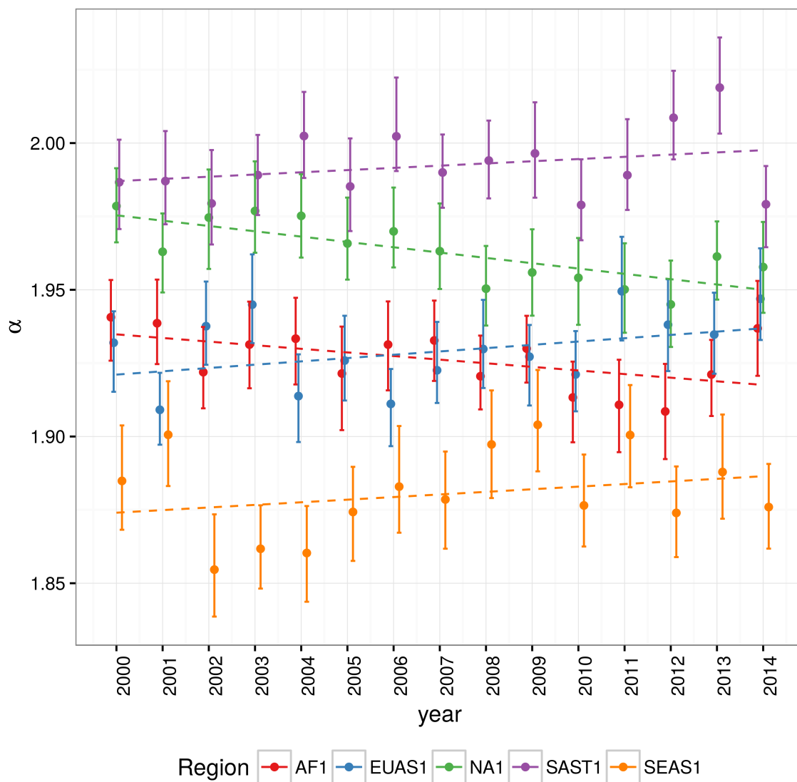
Figure 2: Power law exponents ( \alpha ) of forest patch distributions for regions with total forest area > 10^7 km 2 . Dashed horizontal lines are the fitted generalized least squares linear model, with 95% confidence interval error bars estimated by bootstrap resampling. The regions are AF1: Africa mainland, EUAS1: Eurasia mainland, NA1: North America mainland, SAST1: South America subtropical and tropical, SEAS1: Southeast Asia mainland. For EUAS1 the best model is log-normal but the exponents are included here for comparison.
