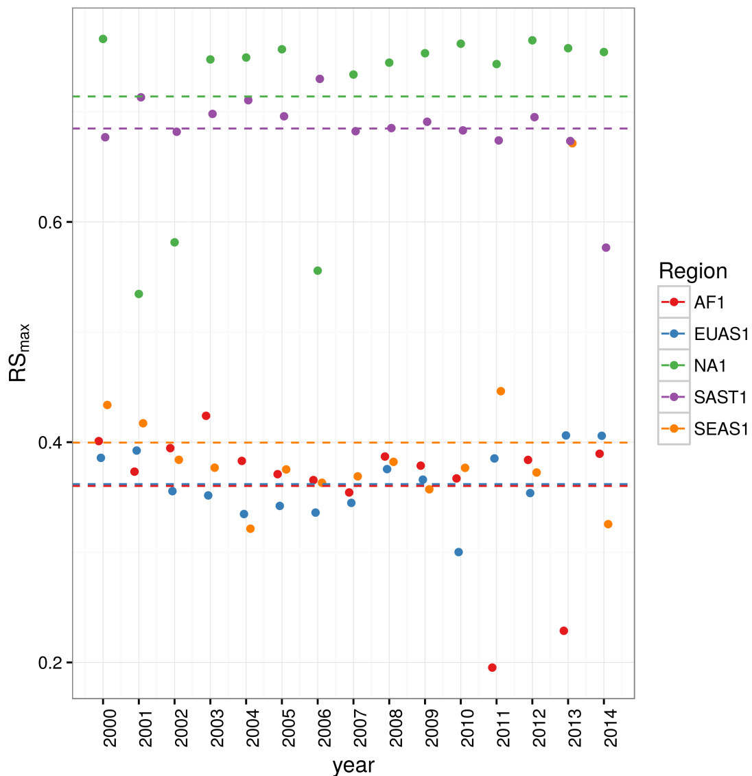
Figure 3: Largest patch proportion relative to total forest area RS_{max} , for regions with total forest area > 10^7 km 2 . Dashed lines are averages across time. The regions are AF1: Africa mainland, EUAS1: Eurasia mainland, NA1: North America mainland, SAST1: South America tropical and subtropical, SEAS1: Southeast Asia mainland.
