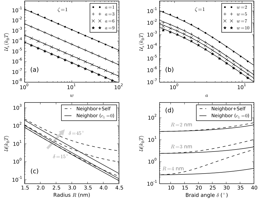
FIG. 6. (a) Comparison of numerical evaluation (points) of \mathcal{U}_s (Eq. A.3) with the proposed empirical solution (Eq. A.4) (solid lines) with \zeta = 1 , c_1 = 0.042 and c_2 = 0.312 , as a function of w for various values of a = 1, 3, 6 and 9 . (b) \mathcal{U}_s versus a for w = 2, 5, 7 and 10 showing that the empirical function is a good fit to the numerical solution. (c) Plot of the total electrostatic potential \mathcal{U} per unit braid length A (Eq. A.5) with (dashed lines) and without (solid lines) the self interaction component (the second term in Eq. A.5 containing the self interaction can be set to zero by putting c_1 = 0 ) versus braid radius ( R ) over a range of braiding angles \delta = 15^\circ, 30^\circ and 45^\circ (Table I). We used \zeta = 2700 (corresponding to 100 mM \text{Na}^+ , Table I), c_2 = 0.312 and c_1 was chosen to be either 0 (only neighbor interaction plot, solid lines) or 0.042 (neighbor and self interaction plot, dashed line). (d) Comparison of the self and the neighbor components of the total electrostatic potential as a function of braiding angle \delta for braid radii R = 2, 3 and 4 nm. The self-energy contribution is non-negligible in braids with radii \gtrsim 3 nm, which is the case \lesssim 2 pN at 100 mM salt (Figure 7a).
