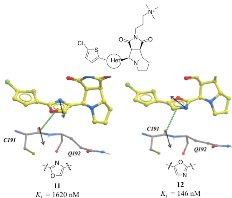
Figure 9. X-ray cocrystal structure of 11 (PDB: 2Y5H) and 12 (PDB: 2Y5G) bound at the active site of factor Xa. The amide \cdots\pi stacking interaction is shown as dotted green lines. The dipoles of the oxazole ring and peptide amide (black arrows) are parallel in 11 and anti-parallel in 12 .
