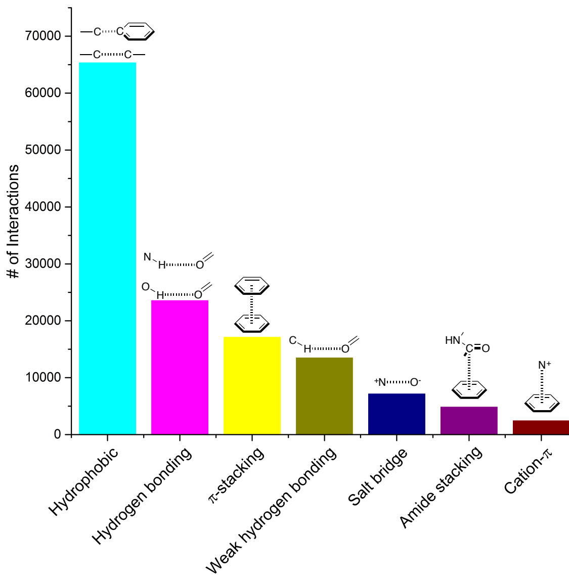
Figure 1. Frequency distribution of the most common non-covalent interactions observed in protein-ligands extracted from the PDB.
