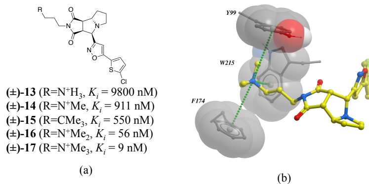
Figure 10. a) Chemical structure of a series inhibitors of human factor Xa; b) in the X-ray cocrystal structure of human factor Xa and 17 (PDB: 2JKH), the quaternary ammonium ion fill the aromatic box. The cation- \pi interaction is displayed as dotted green lines.
