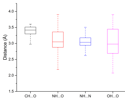
Figure 4. Box plots of hydrogen bond length distributions for the weak (C-H...O) and strong hydrogen bonds (N-H...O, N-H...N, O-H...O).
