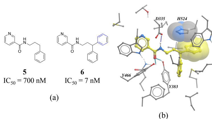
Figure 6. a) Chemical structure of two inhibitors of human sEH; b) X-ray cocrystal structure of human sEH and 6 (yellow carbons, PDB: 3I1Y), the phenyl ring is positioned to allow a \pi -stacking interaction with H524. Hydrogen bonds are displayed in dotted green lines.
