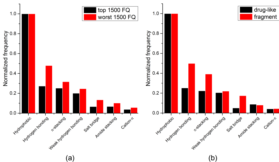
Figure 2. Relative frequency distribution of the most common non-covalent interactions observed in: (a) ligands with high vs. low ligand efficiency; (b) fragments vs. drug-like compounds.
