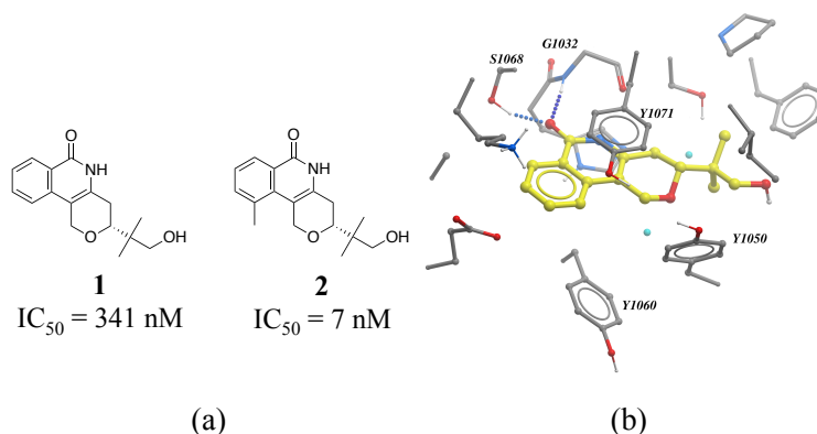
Figure 3. Magic methyl effect: (a) Chemical structure of two TNKS2 inhibitors; (b) crystal structure of 1 (carbon atoms in yellow) bound to TNKS2 (PDB: 5C5P). Oxygen atoms are in red (cyan for water molecules).
