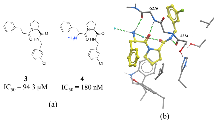
Figure 5. Effect of adding a hydrogen bond in a thrombin inhibitor: a) chemical structure of a pair of thrombin inhibitors; b) crystal structure of 4 (yellow carbons) in complex with thrombin (PDB: 2ZC9). Hydrogen bonds are displayed in dotted green lines and waters oxygens as cyan.
