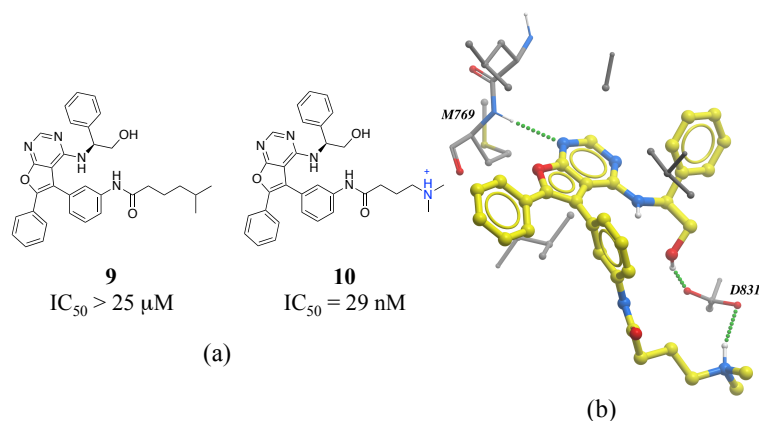
Figure 8. a) Chemical structure of two inhibitors of human EGFR; b) X-ray cocrystal structure of kinase domain of EGFR and 10 (PDB: 4JRV), the terminal N,N -dimethylamino tail of 10 forms a salt bridge with D831. Hydrogen bonds are displayed in dotted green lines.
