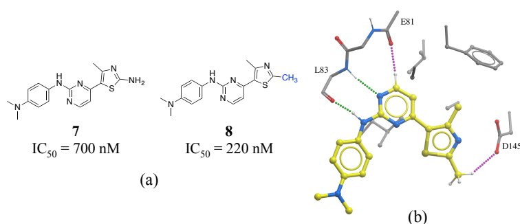
Figure 7. a) Chemical structure of two CDK2 inhibitors; b) X-ray cocrystal structure of human CDK2 and 8 (PDB: 1PXP). The N-H...O and C-H...O hydrogen bonds are displayed as green and magenta dotted lines, respectively.
