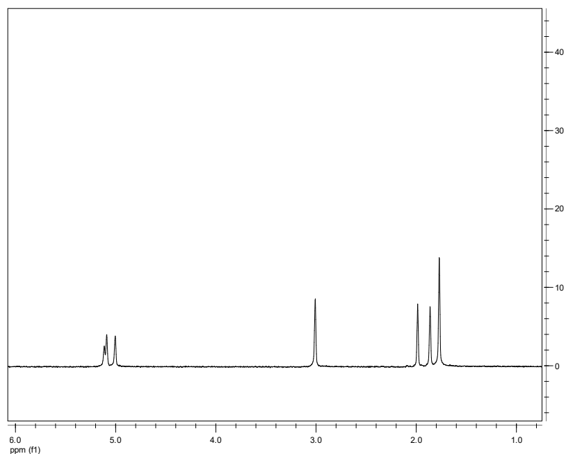
Figure 1. Deuterium NMR spectrum of methallylcyanide- d_7 , an equilibrium mixture of 3-methyl-2-butenitrile- d_7 and 3-methyl-3-butenitrile- d_7 . The predicted boiling points of these two components are within 2 °C, thus these isomers cannot be separated by fractional distillation.
