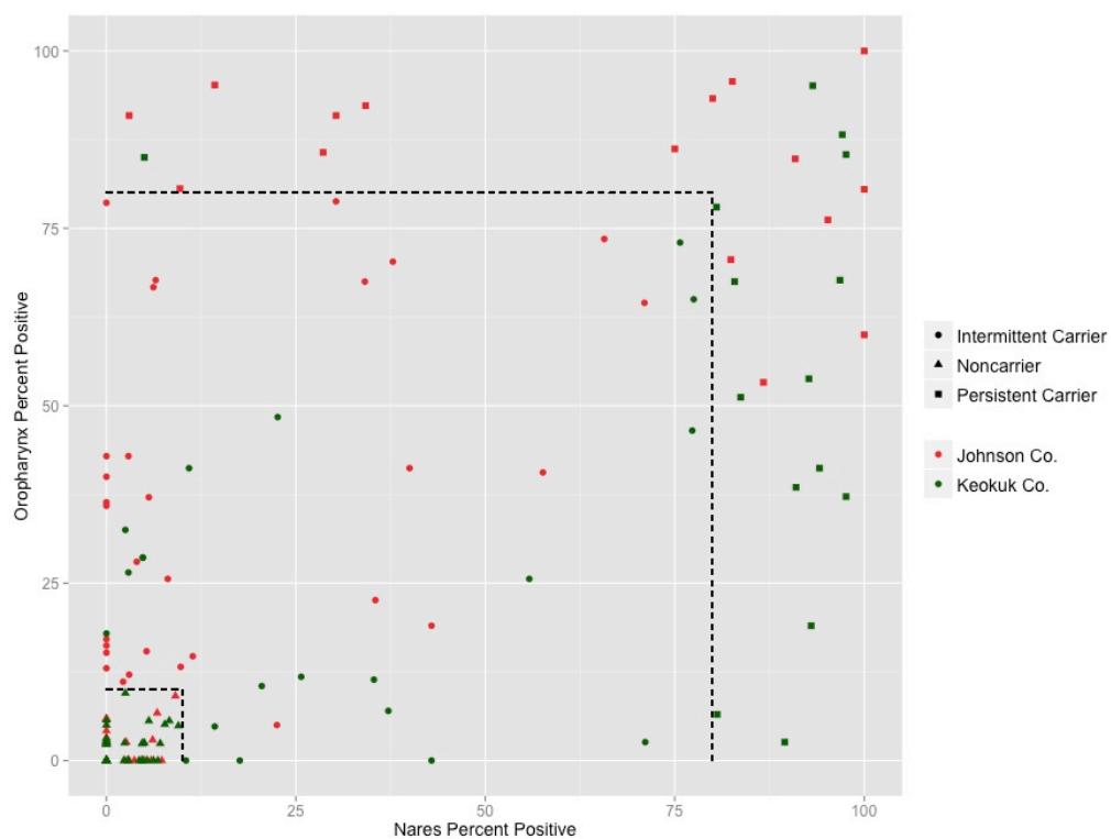
Figure 1: Scatterplot of participant nares and oropharynx colonization rates. Each circle denotes a single participant. Black-dashed lines indicate cutoffs between non-carriers, intermittent carriers, and persistent carriers (21).
