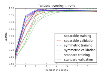
Figure 3: Models with SFC layer learn in fewer epochs. Learning curves show auROC (averaged across all outputs) for simulated TF-binding dataset for standard model, model with SFC, and model with symmetric SFC.
