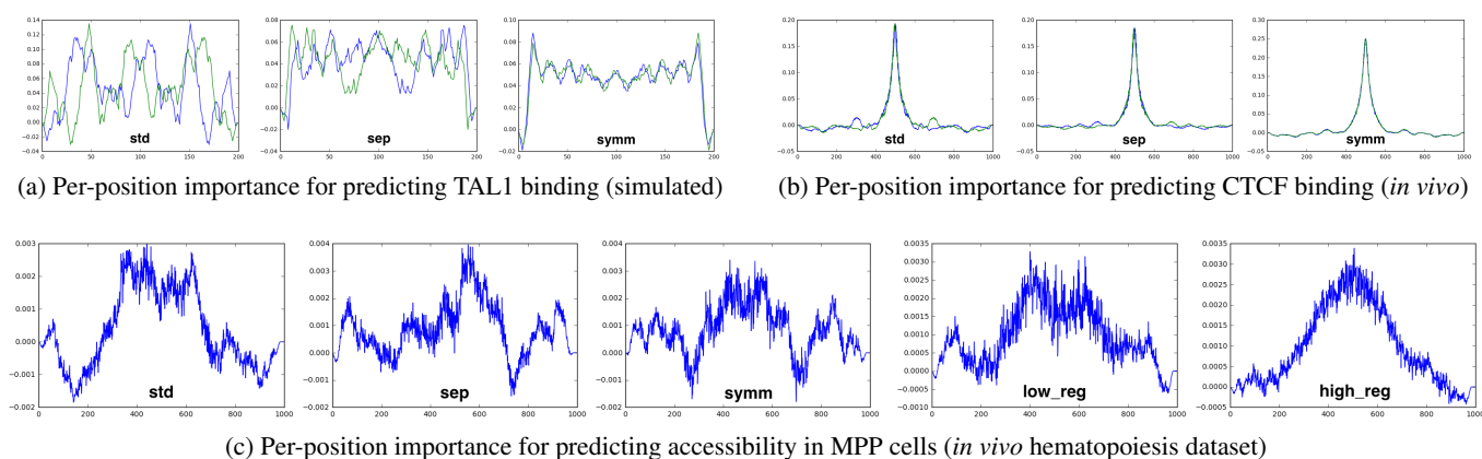
Figure 4: SFC layers improve per-position importance scores. Importance scores were computed on the input sequences using gradient \times input as described in Shrikumar et al. [2017a] for the best performing model over 10 random seeds. Scores at each position were summed across multiple sequences and visualized. Blue lines represent the original per-position importance. Green lines in a and b are mirror images of the corresponding blue lines (they are included to aid with visually assessing symmetry). std is standard model, sep is model with SFC, symm is model with SFC and symmetry constraint (see Sec. 2.4). a : per-position scores TAL1 task in simulated TF-binding, averaged over 100K generated sequences. b : per-position scores for in-vivo CTCF task, averaged over regions in the testing set. c : per-position scores for MPP accessibility task in hematopoiesis dataset, averaged over 10K regions. low_reg has CR=1.0 and high_reg has CR=10.0 (both have a symmetry constraint).
