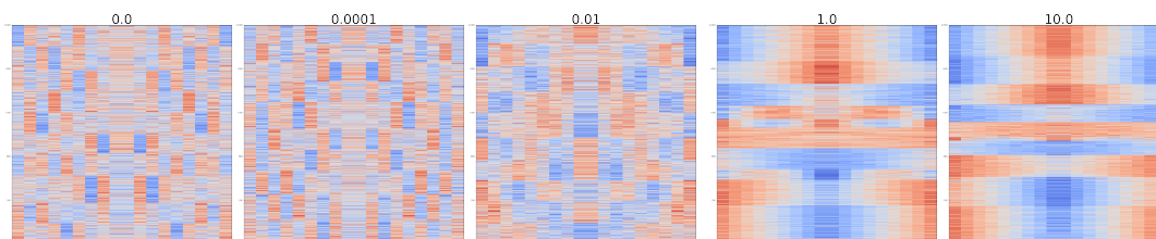
Figure 5: Curvature Regularization produces smoother W_{pos} . Weights of W_{pos} for models trained on hematopoiesis dataset with different levels of CR are visualized. Each row corresponds to a single output neuron. Strength of CR is indicated on the top. Rows were mean-normalized to have unit magnitude, and clustered using k-means clustering with k = 10 . Symmetry was enforced for all models.
