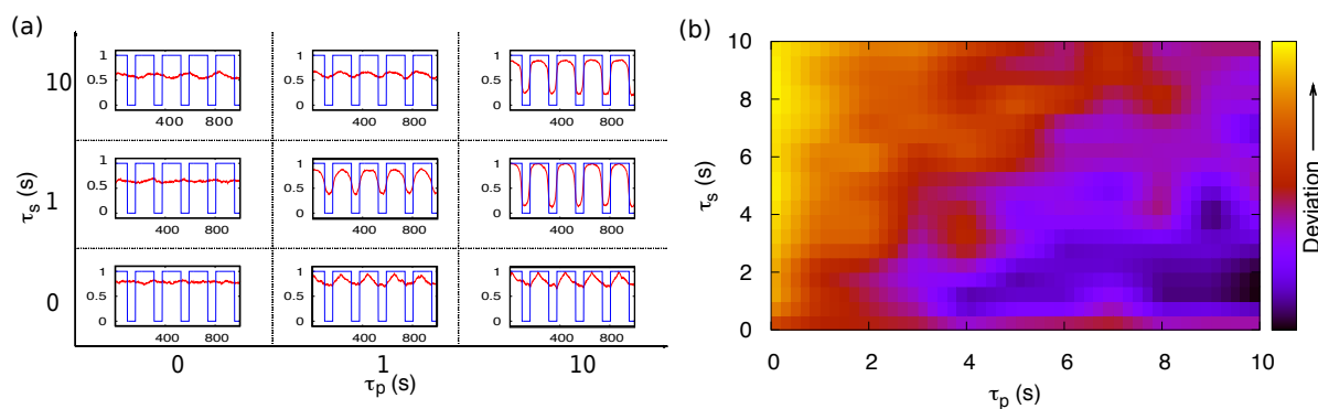
Figure 3: Comparison of nucleosome organization between parent and daughter chromatin for various pairs of (\tau_p, \tau_s) values. (a) Blue sharp curves represent the parental nucleosome organization and the red curves represent daughter nucleosome organization averaged over an ensemble of realizations. (b) Heat-map for the quantity ‘deviation’ ( \chi ) as defined in eq. 1, \chi increases as color varies from violet to yellow. For 0 < \tau_s \leq \tau_p there is less deviation from parent to daughter nucleosomal organization.
